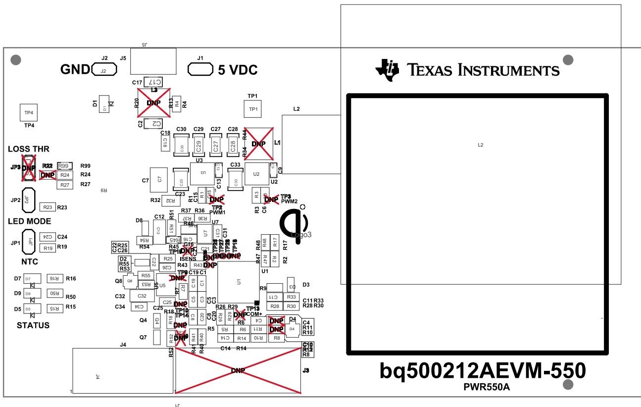
Figure 6. Assembly Top
