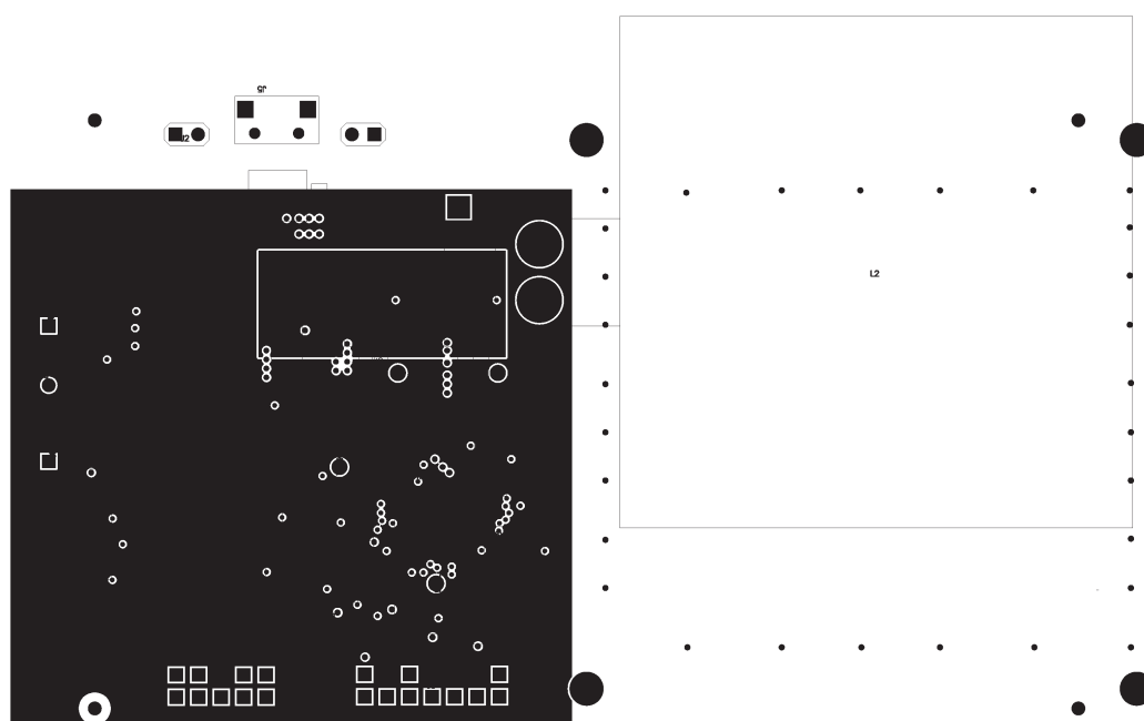
Figure 9. Layer 2
